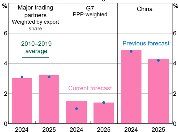
Graph 3.1 GDP Growth Year-average
