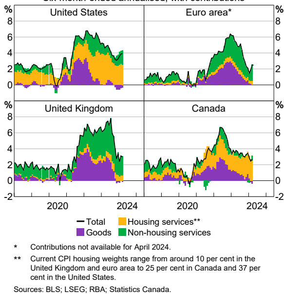
Graph 2.5 Core Consumer Price Inflation Six-month-ended annualised, with contributions
