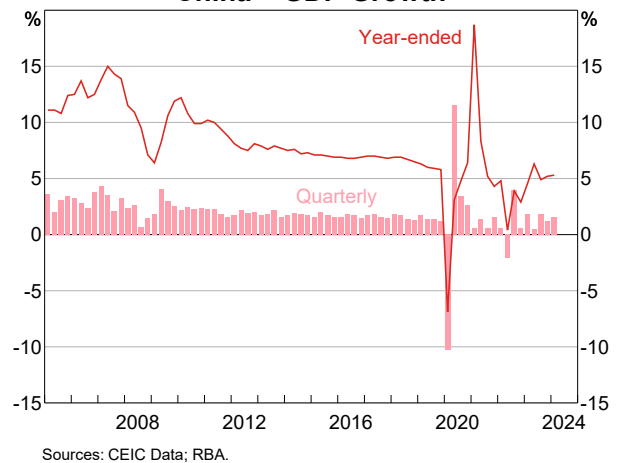
Graph 2.7 China – GDP Growth
