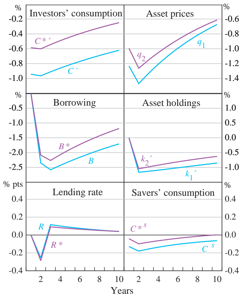
Figure 7: Low Leverage Constraints, Partial Diversification
