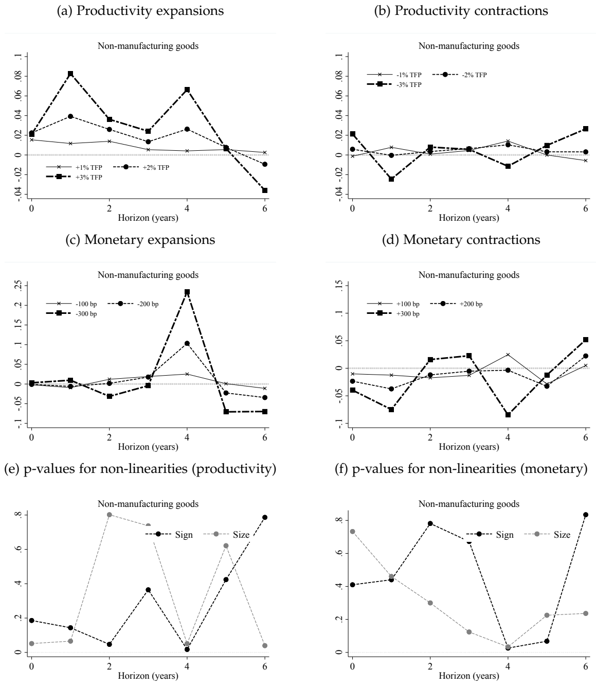
Figure 12: Non-linear IRFs of intermediates intensity to productivity and monetary shocks
