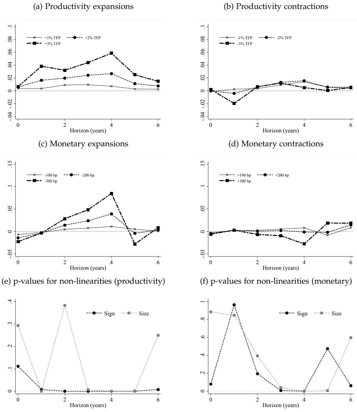
Figure 9: Non-linear IRFs of intermediates intensity to productivity and monetary shocks
