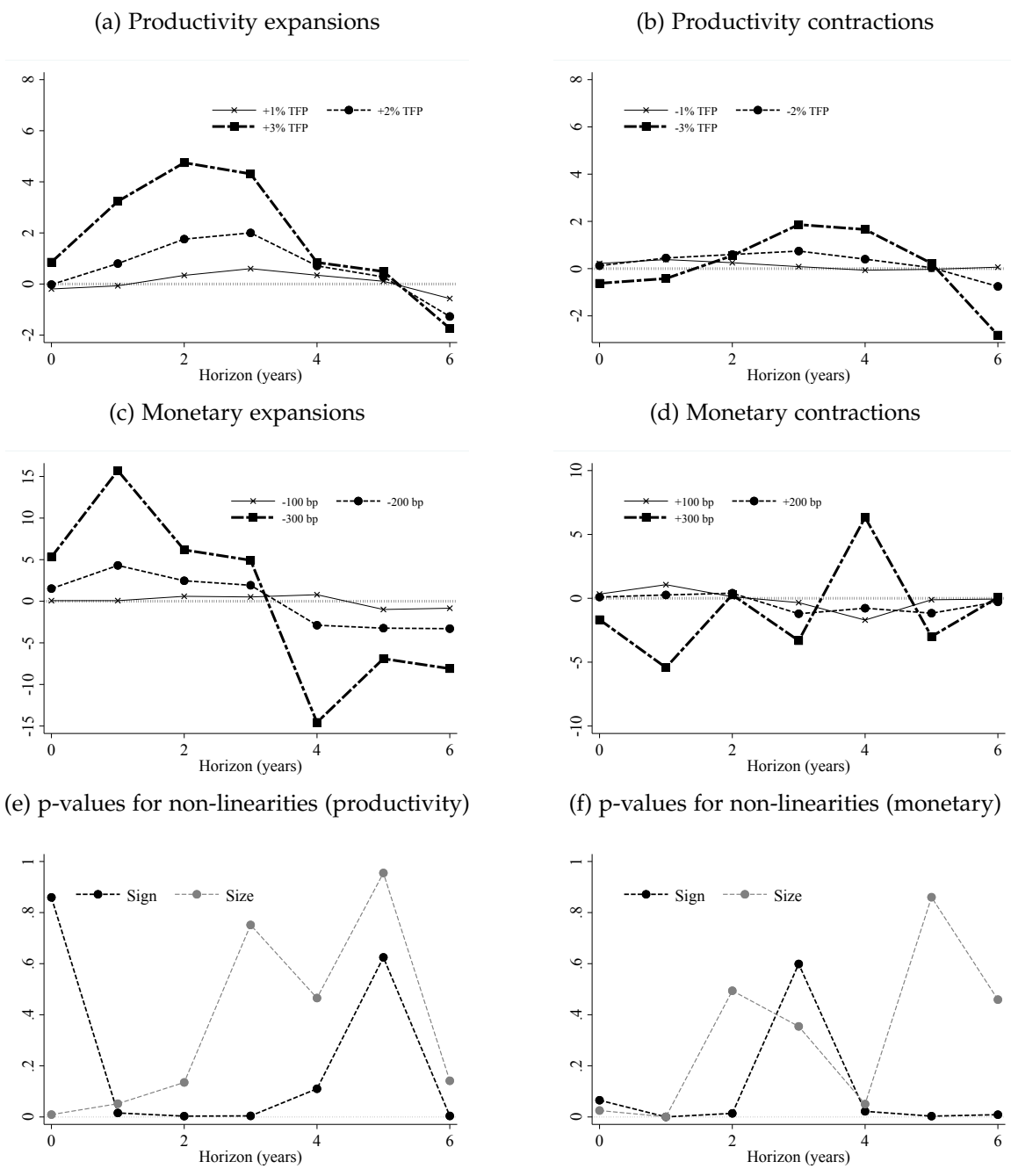
Figure 19: Non-linear IRFs of number of suppliers to productivity and monetary shocks
