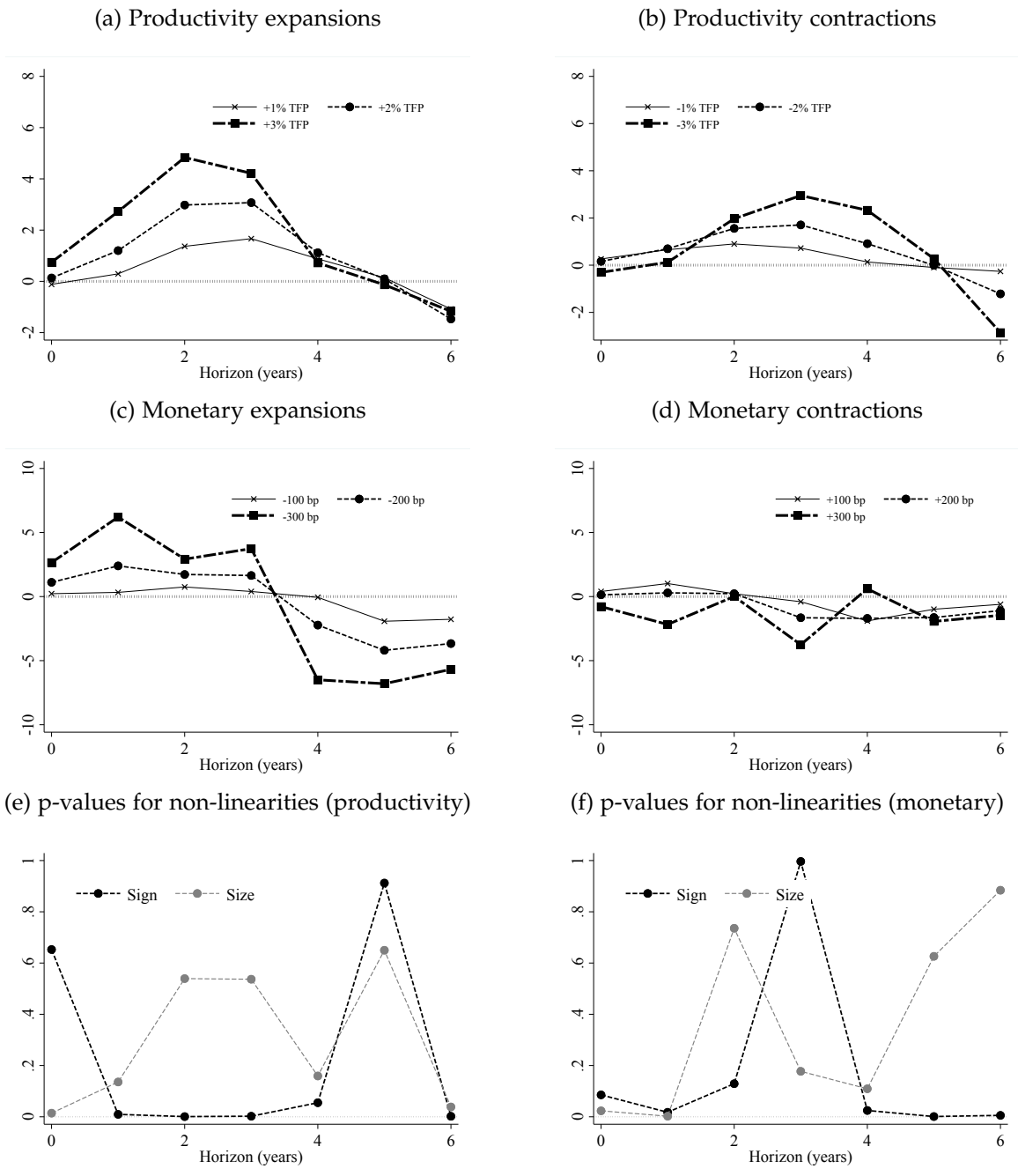
Figure 11: Non-linear IRFs of number of suppliers to productivity and monetary shocks
