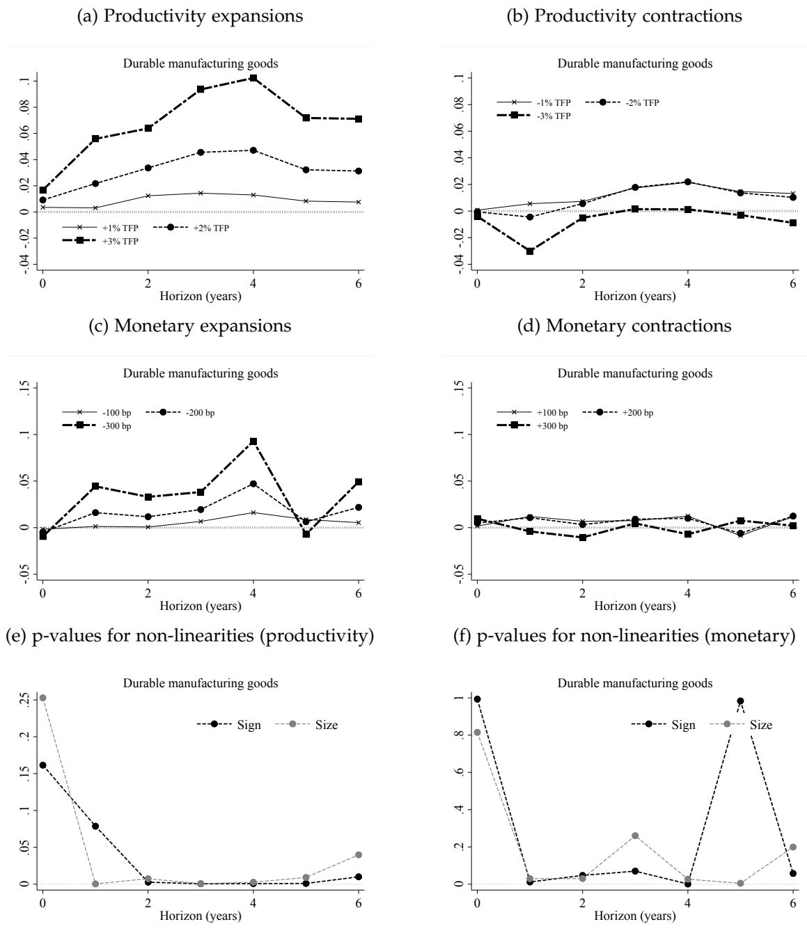
Figure 13: Non-linear IRFs of intermediates intensity to productivity and monetary shocks
