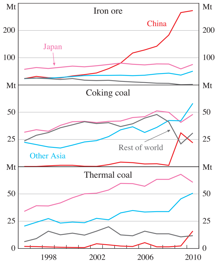
Figure 12: Bulk Commodity Export Volumes
