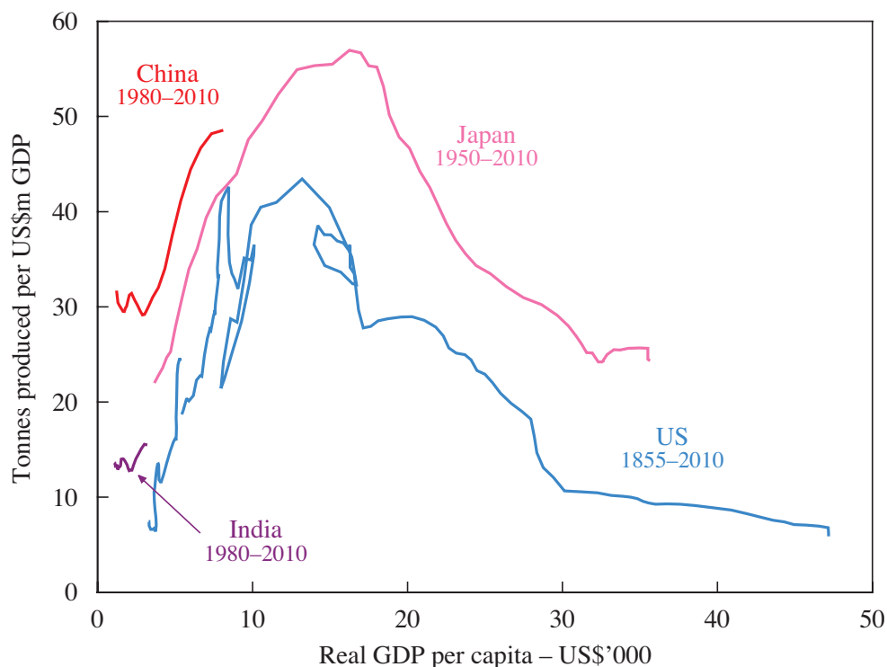
Figure 6: Steel Production Intensity and Economic Development
