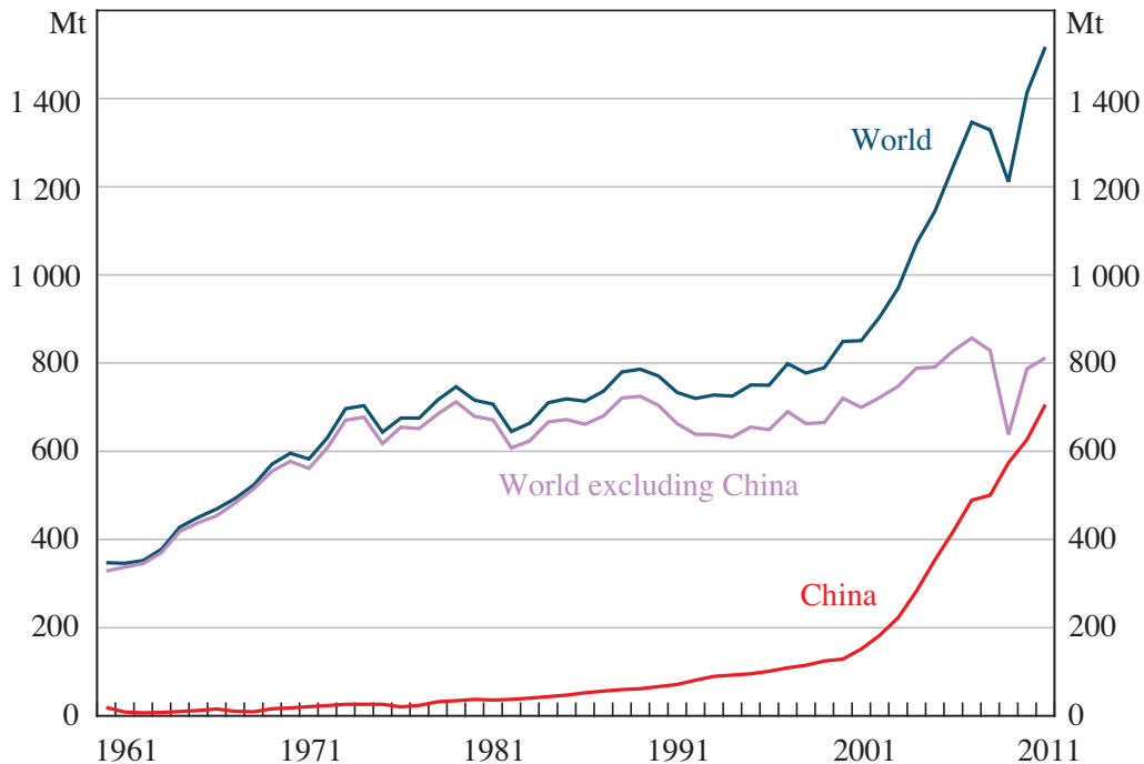
Figure 4: World Steel Production
